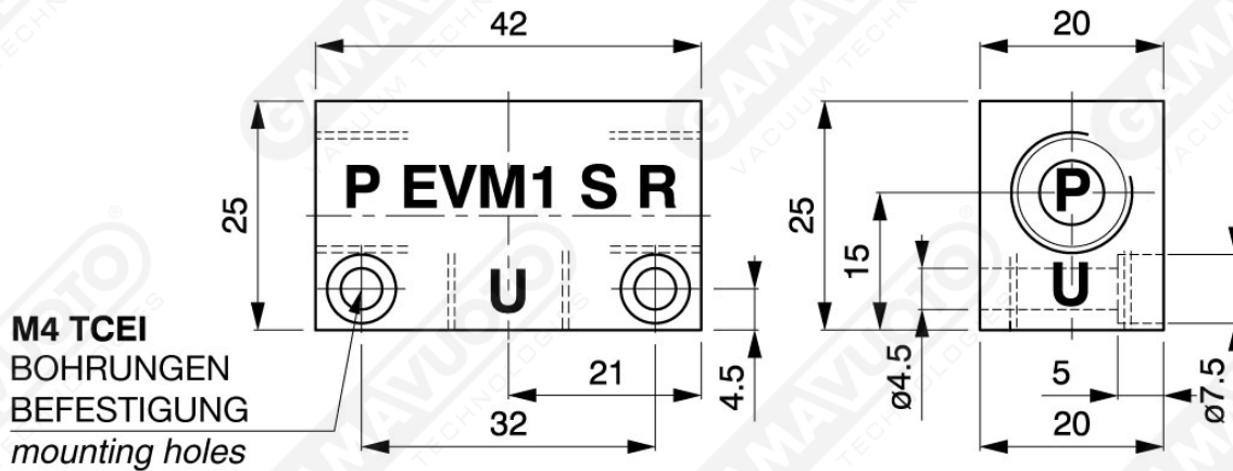
Art. EVM1SC
