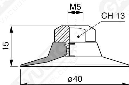
Art. EF 40 90 ÷ 93
