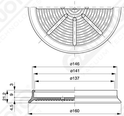
Art. VDO 160
