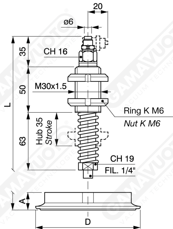
Art. PMD 90/120/160
